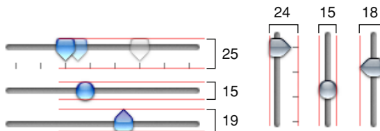
Figure 14-33 Full-size slider control dimensions
