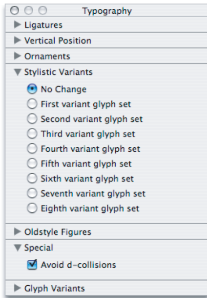
Figure 5-6 Typography inspector
